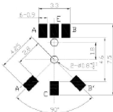
P.C.B.MOUNTING DETAIL
